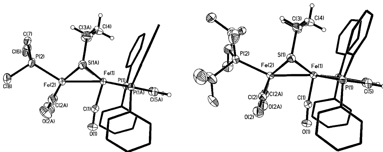
Figure 6. Structure of the cations in [\mathbf{3pdt}]\text{BF}_4 and [\mathbf{5pdt}]\text{BF}_4 with thermal ellipsoids set at 35% level. Phenyl ellipsoids, hydrogen atoms, and the \text{BF}_4^- were omitted for clarity.
