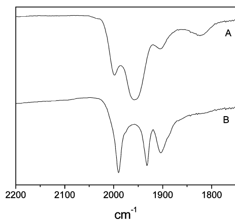
Figure 7. IR spectra (KBr) of [\mathbf{5pdt}]\text{BF}_4 that was rapidly precipitated (A) and of single crystals grown at -20\text{ }^\circ\text{C} (B).
