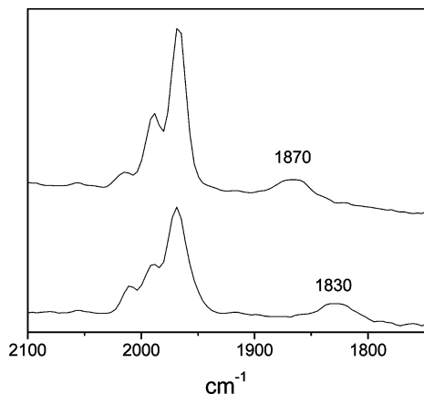
Figure 3. IR spectra (absorbance mode, \text{CH}_2\text{Cl}_2 at -45^\circ\text{C} ) showing the effects of edt vs pdt for the oxidation of complexes containing bulky phosphine ligands: [\text{Fe}_2(\text{S}_2\text{C}_2\text{H}_4)(\text{CO})_3(\text{Pi-Pr}_3)(\text{dppv})]\text{BF}_4 ( [\mathbf{5edt}]\text{BF}_4 , top) and [\text{Fe}_2(\text{S}_2\text{C}_3\text{H}_6)(\text{CO})_3(\text{Pi-Pr}_3)(\text{dppv})]\text{BF}_4 ( [\mathbf{5pdt}]\text{BF}_4 , bottom).
