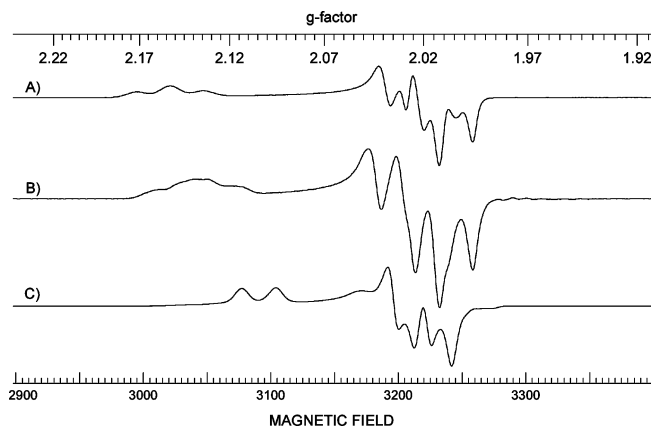
Figure 4. X-Band EPR spectra (110 K, 1:1 \text{CH}_2\text{Cl}_2 :toluene frozen solution): [\text{Fe}_2(\text{S}_2\text{C}_3\text{H}_6)(\text{CO})_4(\text{dppv})]^+ ( [\mathbf{2pdt}]^+ , (A)), [\text{Fe}_2(\text{S}_2\text{C}_3\text{H}_6)(\text{CO})_3(\text{PMe}_3)(\text{dppv})]^+ ( [\mathbf{3pdt}]^+ , (B)), [\text{Fe}_2(\text{S}_2\text{C}_3\text{H}_6)(\text{CO})_3(\text{Pi-Pr}_3)(\text{dppv})]^+ ( [\mathbf{5pdt}]^+ , (C)).
