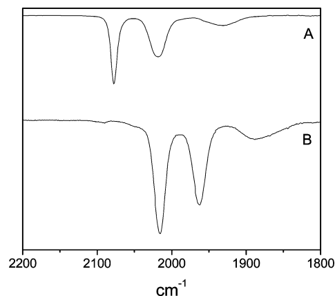
Figure 2. IR spectra (CH 2 Cl 2 solns) of [Fe 2 (S 2 C 3 H 4 )(CO) 4 (dppv)]BF 4 ( 2pdt )BF 4 , A) and [Fe 2 (S 2 C 3 H 6 )(CO) 3 (PMe 3 )(dppv)]BF 4 ( 3pdt )BF 4 , B).
