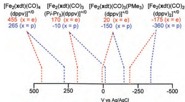
Figure 1. Redox properties of diiron(I) dithiolates (CH 2 Cl 2 soln). Unless indicated otherwise, couples are reversible as judged from the finding that i_{pc}/i_{pa} \sim 1 .
