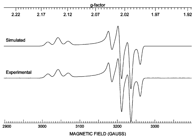
Figure 5. X-Band EPR spectra (110 K, 1:1 CH 2 Cl 2 : toluene frozen solution) of [Fe 2 (S 2 C 2 H 4 )(CO) 3 (PMe 3 )(dppv)]BF 4 ([3edt]BF 4 ). Top is the simulation and bottom is experimental data.
