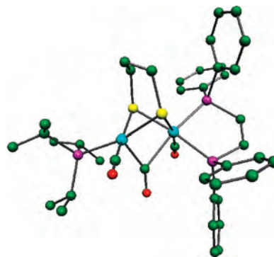
Figure 8. DFT structure of the lowest energy isomer of [\text{Fe}_2(\text{S}_2\text{C}_2\text{H}_4)(\text{CN})(\text{CO})_3(\text{Pi-Pr}_3)(\text{dppv})]^+ ( [\mathbf{5pdt}]^+ ). Atoms are color coded as follows: carbon, green; oxygen, red; sulfur, yellow; phosphorus, purple; iron, cyan.
