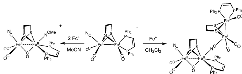
Scheme 5. Redox Reactivity Proposed for [\text{Fe}_2(\text{S}_2\text{C}_2\text{H}_4)(\text{CN})(\text{CO})_3(\text{dppv})]^-
