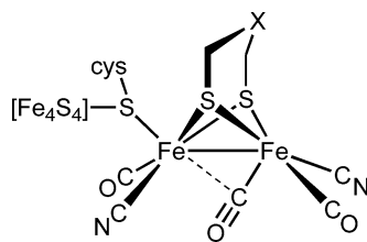
Scheme 1. Structure of the Diiron Active Site of the H ox State of the [FeFe]-Hydrogenases a
